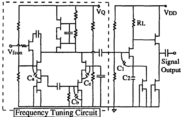
Fig. 5. Circuit diagram of the proposed VCO.
