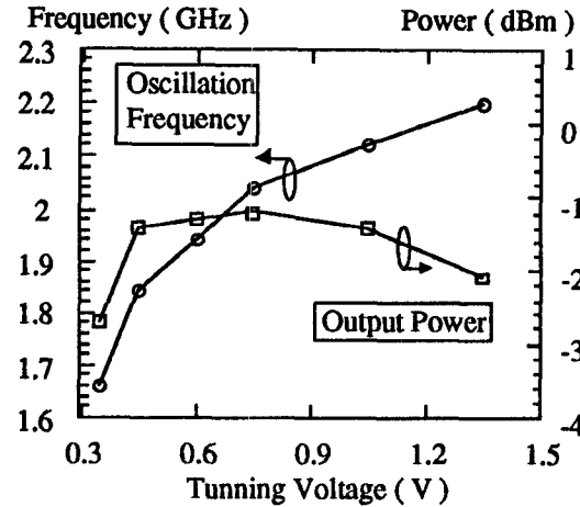
Fig. 6. Simulated performances of the VCO.
